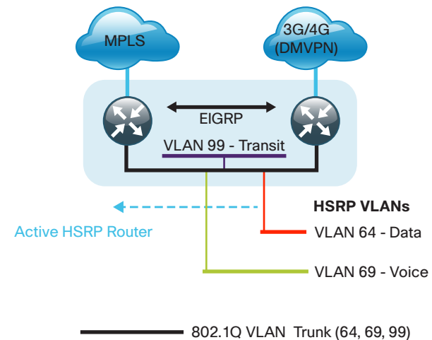
Figure 3 - WAN remote site—flat Layer 2 LAN (dual router)
