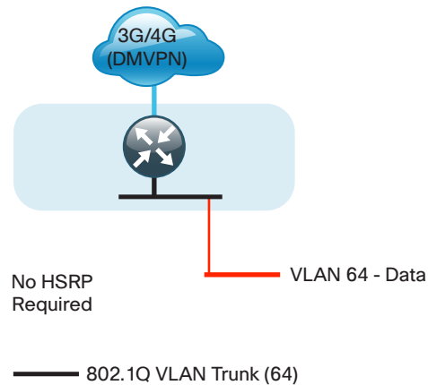
Figure 2 - WAN remote site—flat Layer 2 LAN (single router)
