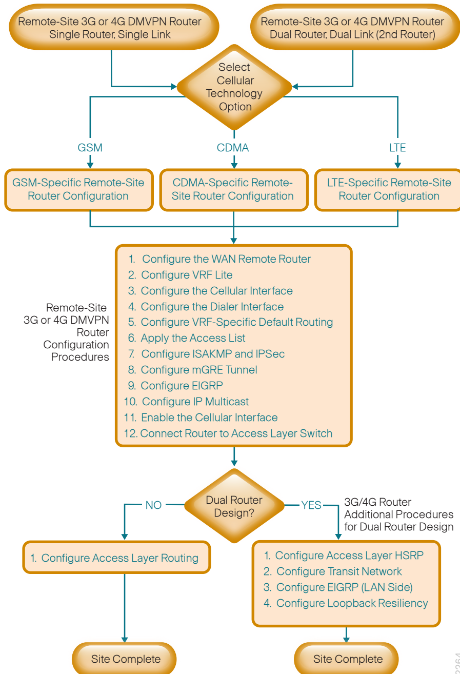
Figure 8 - Flowchart for remote-site 3G or 4G DMVPN spoke router configuration
