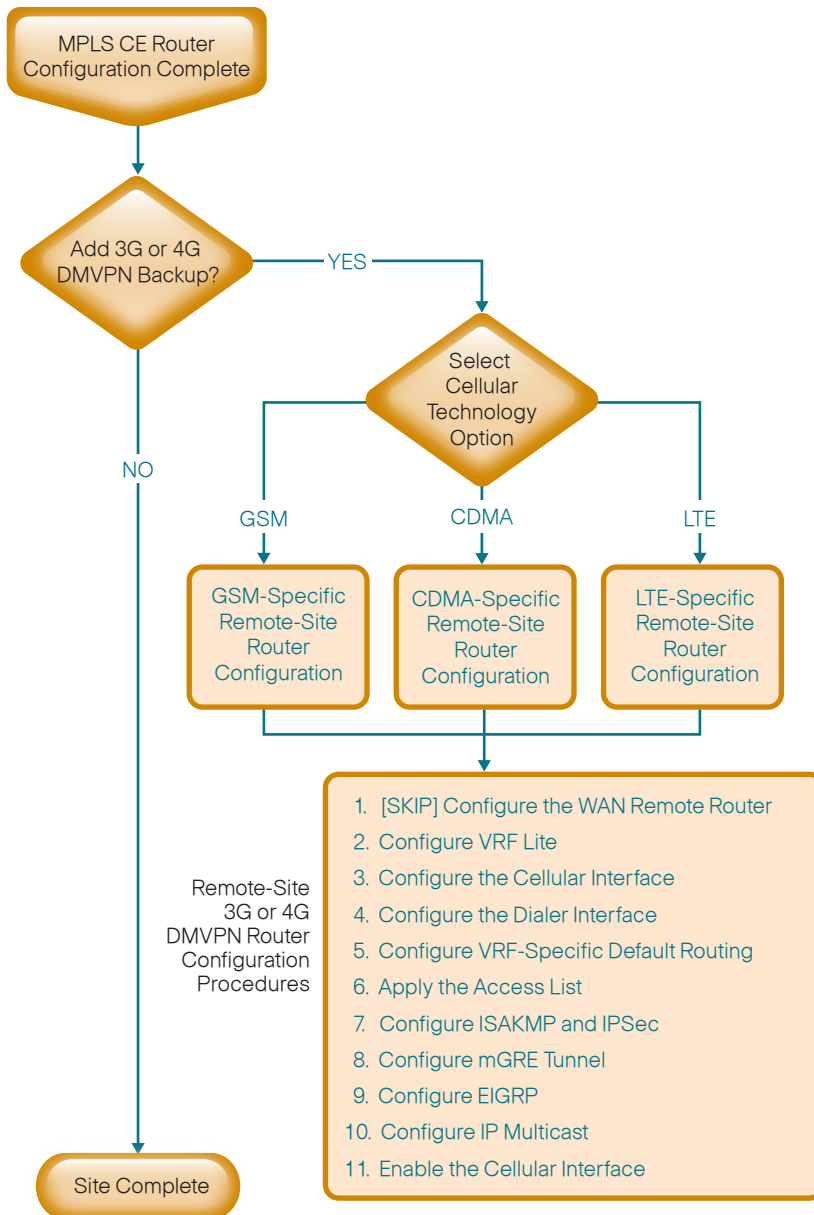
Figure 9 - Flowchart for adding 3G or 4G DMVPN backup to an existing remote-site router configuration
