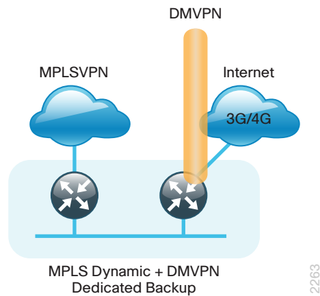
Figure 7 - MPLS WAN + DMVPN remote site (dual router - dual link options)
