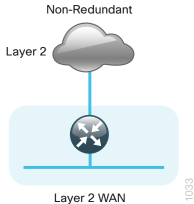
Figure 3 - WAN remote-site design
