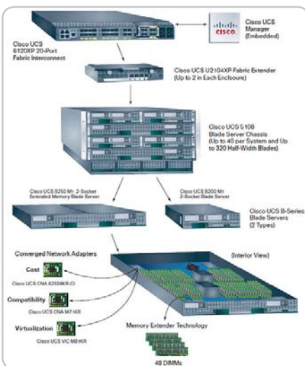
Individual components of the Cisco UCS
