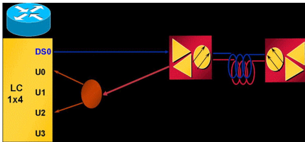
Figure 3 Frequency Stacking
