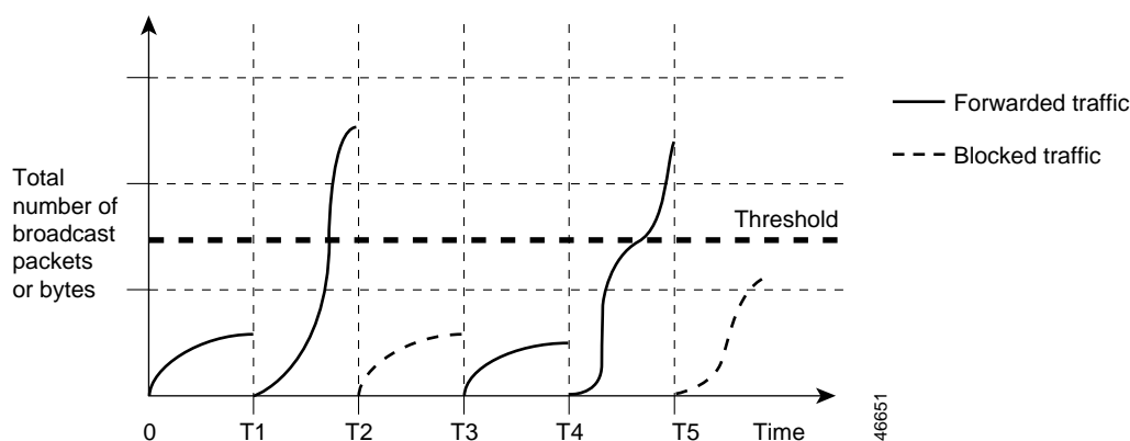
Figure 1-1 Broadcast Storm Control Example
