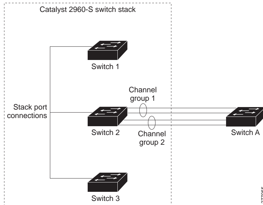
Figure 1-2 Single-Switch EtherChannel
