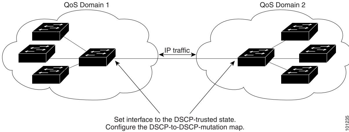
Figure 34-12 DSCP-Trusted State on a Port Bordering Another QoS Domain
