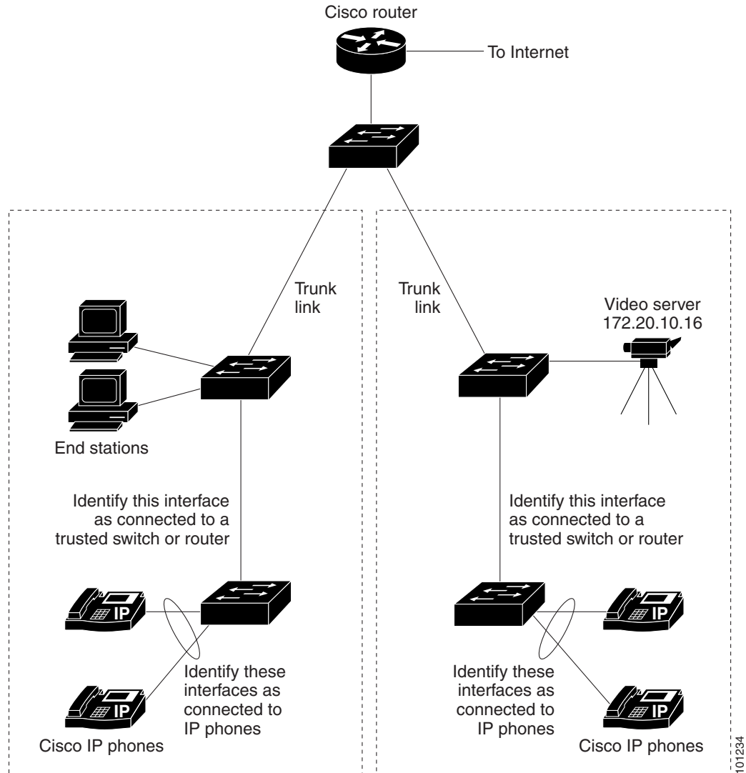
Figure 34-10 Auto-QoS Configuration Example Network
