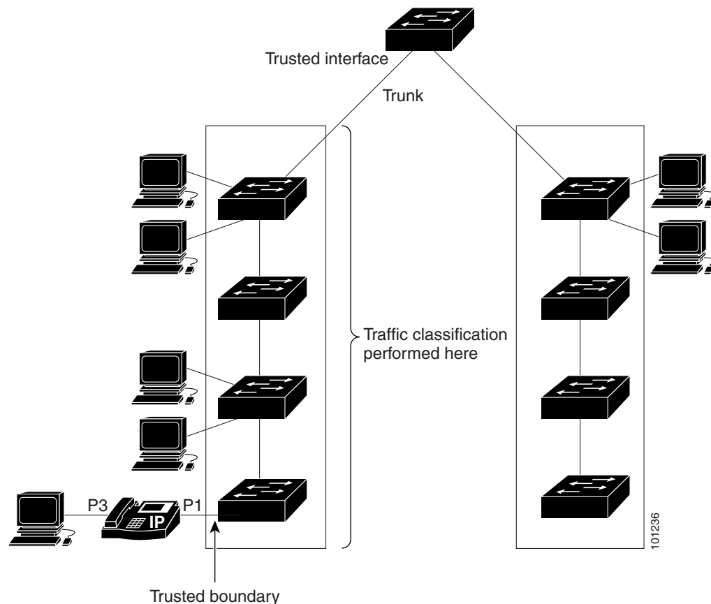
Figure 34-11 Port Trusted States within the QoS Domain
