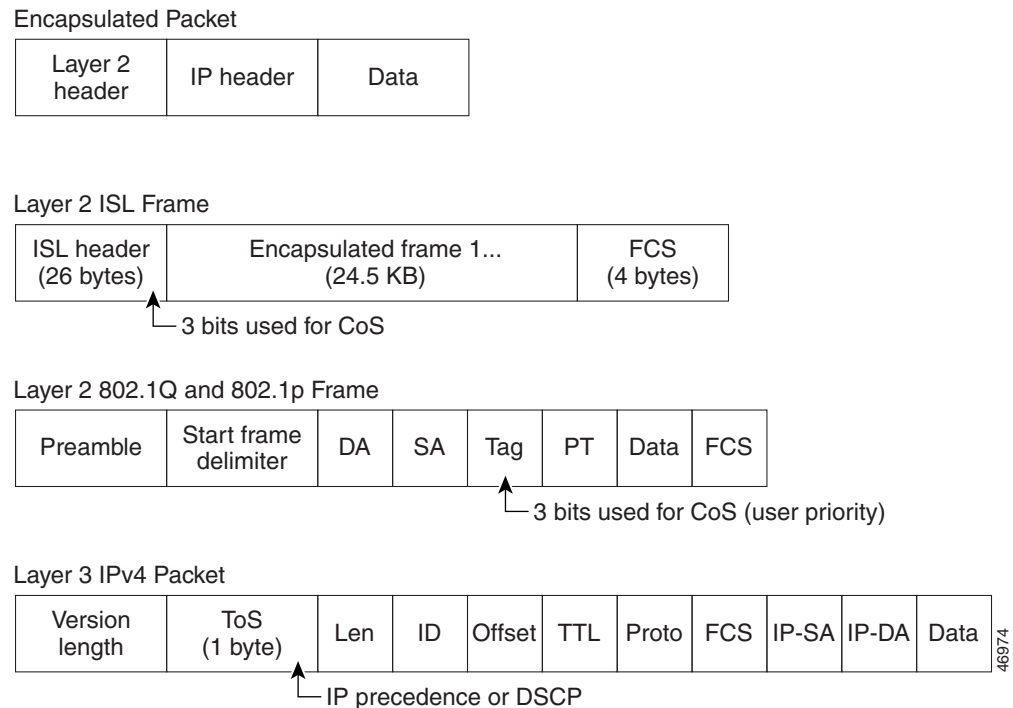
Figure 31-1 QoS Classification Layers in Frames and Packets
