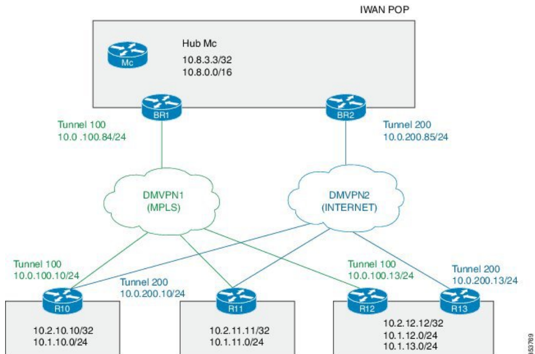
Figure 2: PfRv3 Topology
