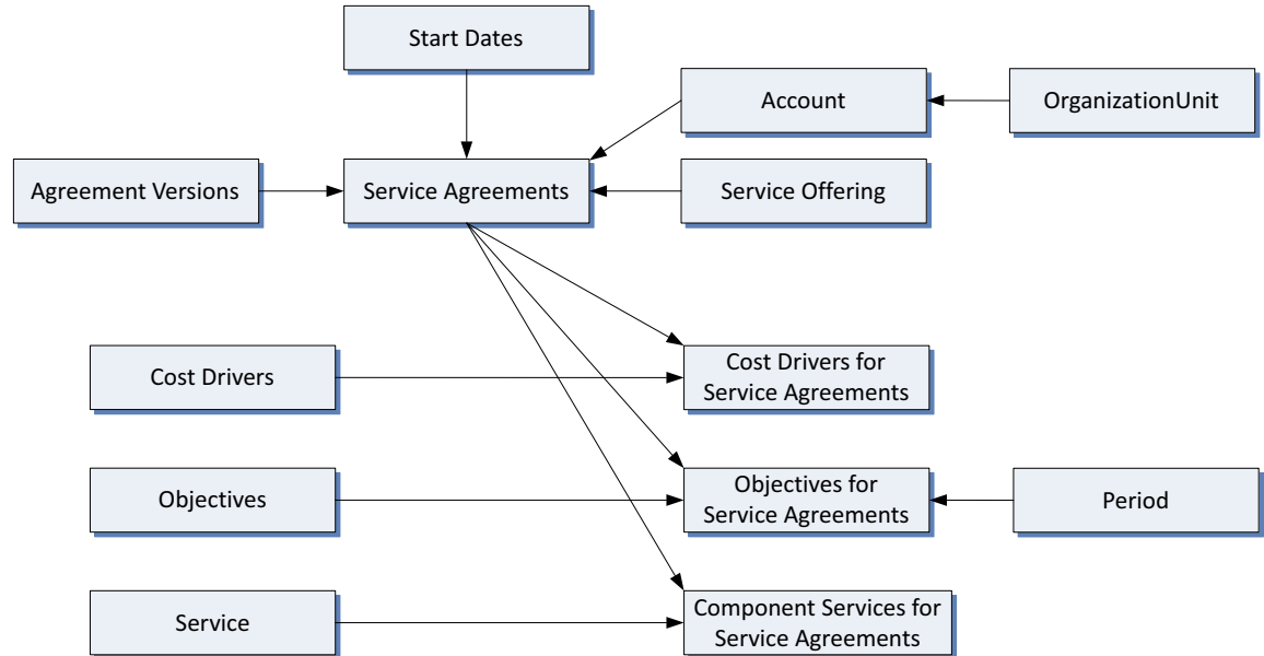
Figure 1-4 Service AGREEMENT Star Schema Diagram
